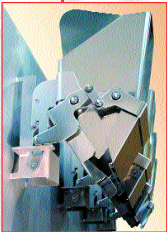
Washrack holds hopper doors open for easy cleaning and complete draining.
