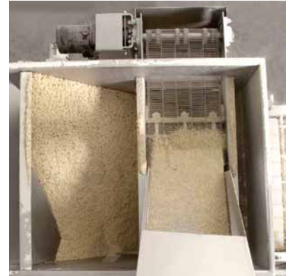
Sifter conveyor removes lumps from non free-flowing breading hopper.
