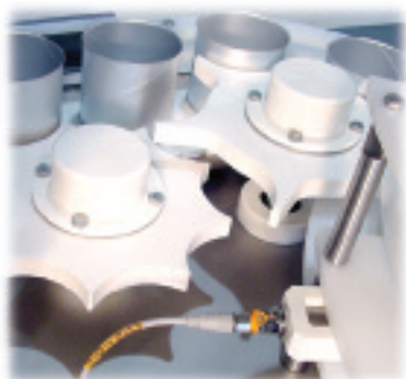
Funnel and starwheels are simply changed for different container sizes.
