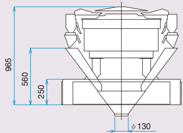
20-head CCW-R-220W-S/08
