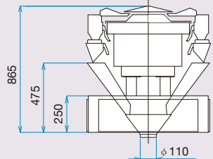
10-head CCW-R-210W-S/08
