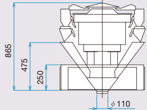
14-head CCW-R-214W-S/08
