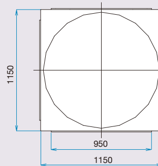
20-head CCW-R-220W-S/08
