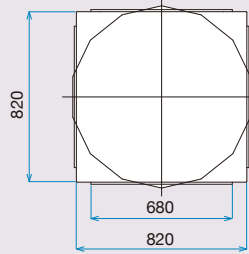
14-head CCW-R-214W-S/08
